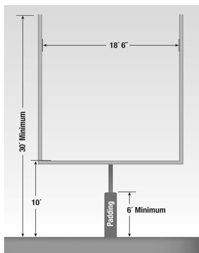
GOAL POST DETAIL
